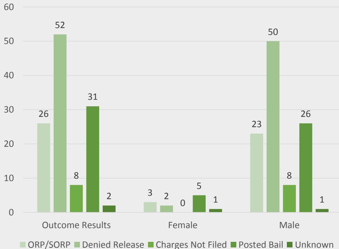
119 Outcomes
